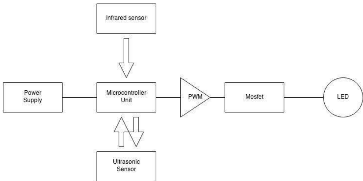
Figure 34: Block diagram
