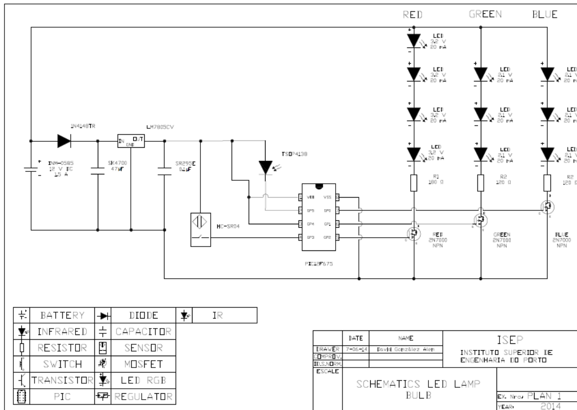
Figure 35: Led driver schematics
