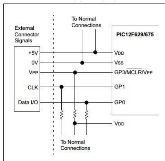
Figure 54: Microcontroller programming [72]
