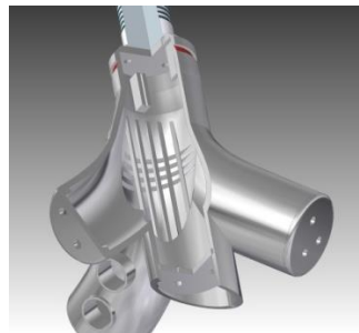
Figure 56: Inner design
