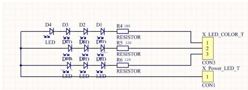
Figure 36: LED panel
