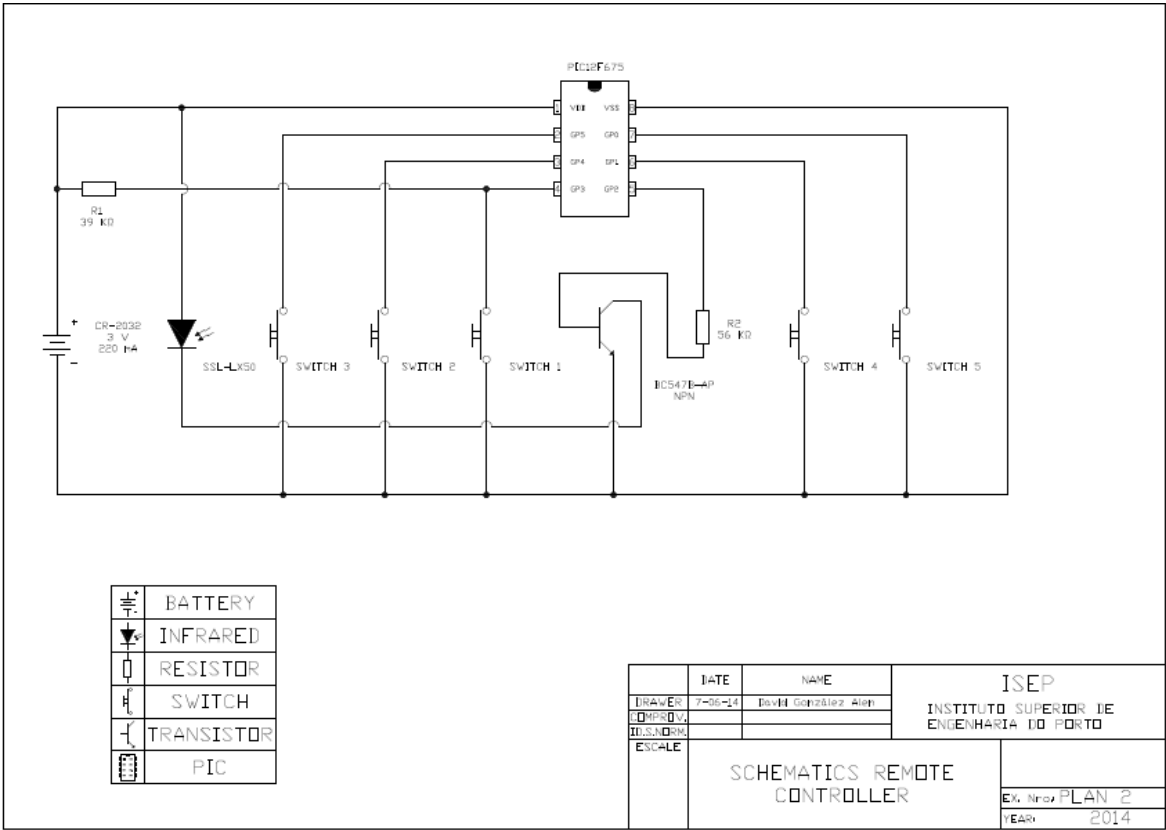
Figure 37: Remote Control schematics
