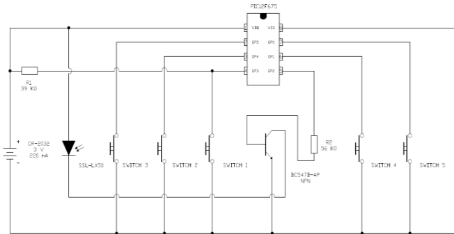
Figure 2: Remote control electrical scheme
