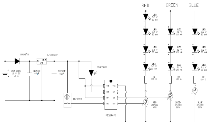
Figure 1: LED Lamp electrical scheme
