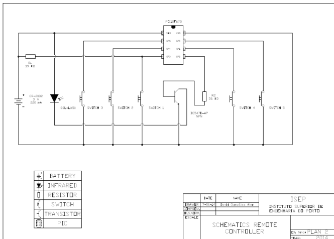
Figure 2: Remote control electrical scheme
